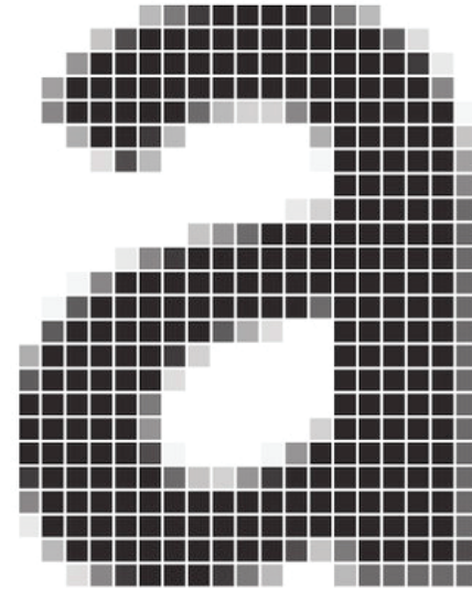
RASTER-BASED GRAPHICS
