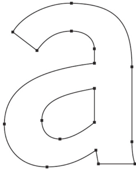
VECTOR-BASED GRAPHICS
